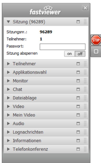
FastViewer Sidebar
